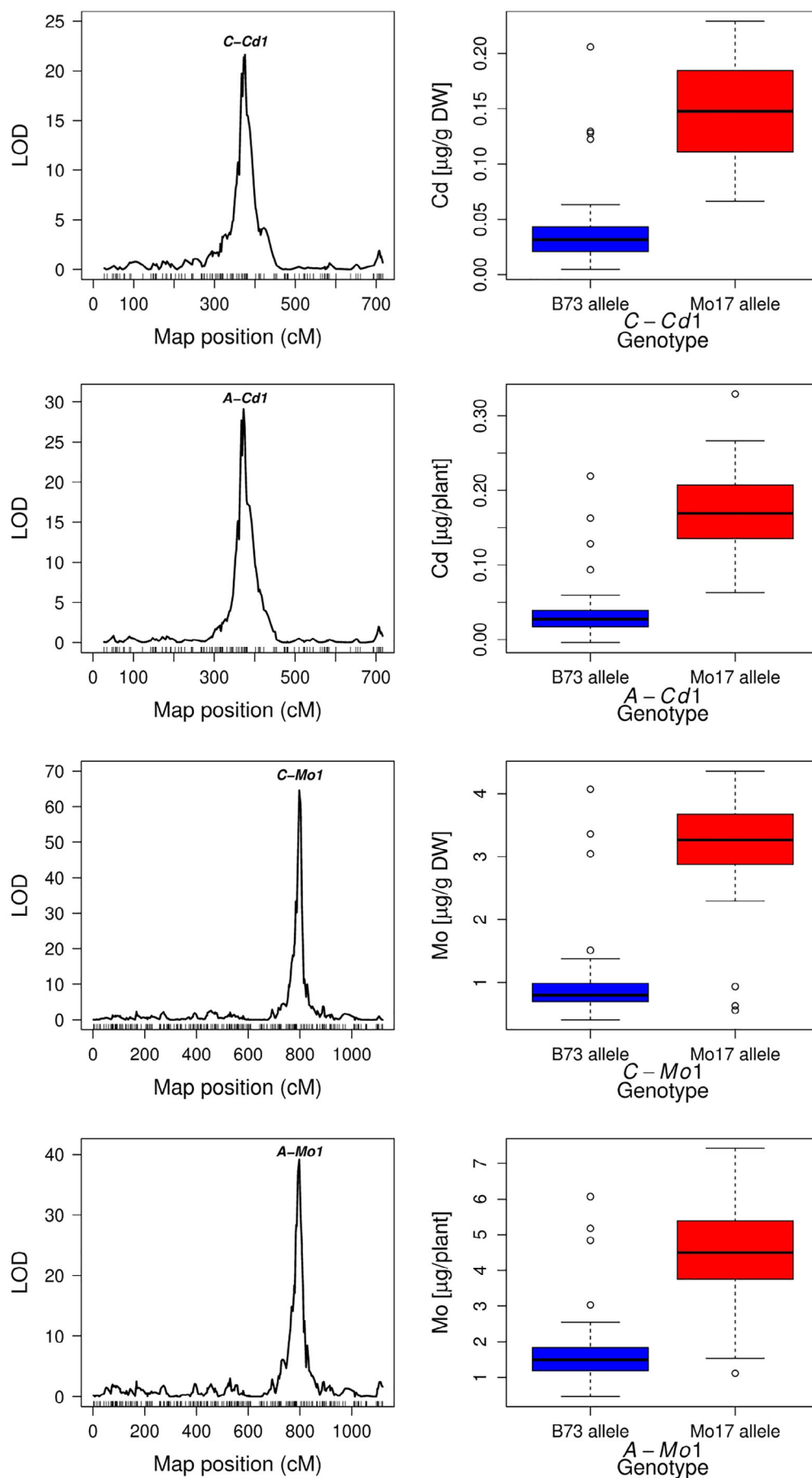
FIGURE 6 The plots in the left column present the logarithm of odds (LOD) versus the position on the genetic map of chromosomes two, two, one, and one, respectively, for a selected set of quantitative trait loci (QTL) with significant main effects across two iron regimes for cadmium (Cd) and molybdenum (Mo) concentration (C-*) and content (A-*) in shoots of the maize IBM population. The plots in the right column are boxplots of the adjusted entry means of the genotypes carrying the B73 or Mo17 allele at the QTL position across the sufficient and deficient Fe regime [Colour figure can be viewed at wileyonlinelibrary.com ]
